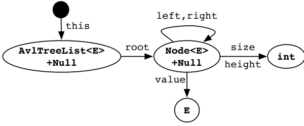
Fig. 5. Type graph for AvlTreeList example.
