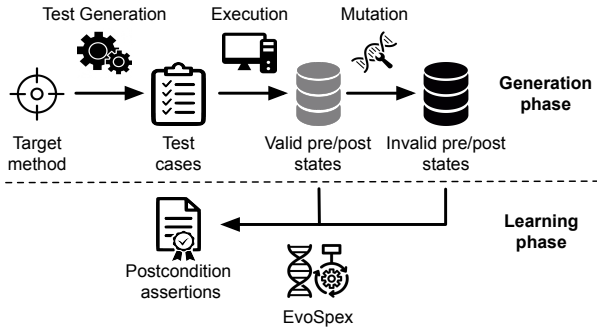
Fig. 4. An overview of the proposed approach
